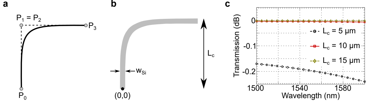
Figure 3.10: a 90^\circ spline bend with knots P_0 and P_3 , and control points P_1 and P_2 . b Cubic spline waveguide 90^\circ bend with width w_{Si} and characteristic length L_c . L_c is measured from the middle of the input waveguide to the edge of the output waveguide (or vice versa). c FDTD simulation of 90^\circ waveguide bend of various characteristic lengths, L_c , for the waveguide shown in Fig. 3.8. For L_c \geq 10 \mu m , simulated bending loss is insignificant across the 1500 nm - 1600 nm range of interest.
