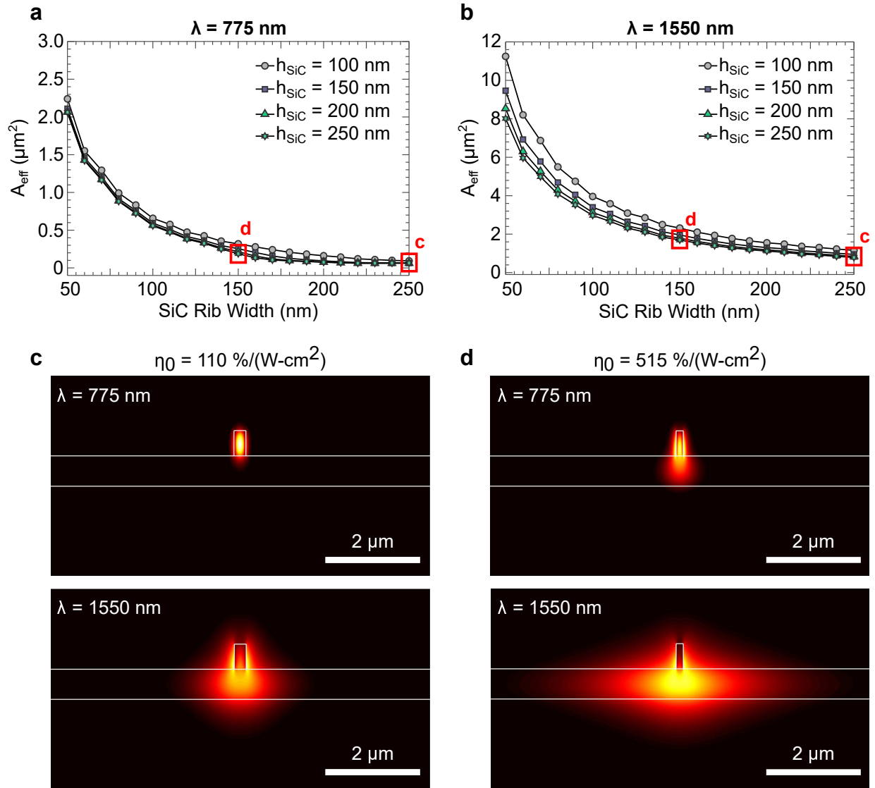
Figure 7.8: Sweep of A_{\text{eff}} versus SiC width at \lambda = 775 nm (part a) and \lambda = 1550 nm (part b) for SiC heights of 100 nm, 150 nm, 200 nm, and 250 nm. c and d show mode pictures for w_{\text{SiC}} = 250 nm and h_{\text{SiC}} = 250 nm (part c) and w_{\text{SiC}} = 150 nm and h_{\text{SiC}} = 250 nm (part d) for the SH mode (top) and the FH mode (bottom). Despite the reduced mode areas of the design of c, the design of d has a higher normalized conversion efficiency due to the locations of the modes.
