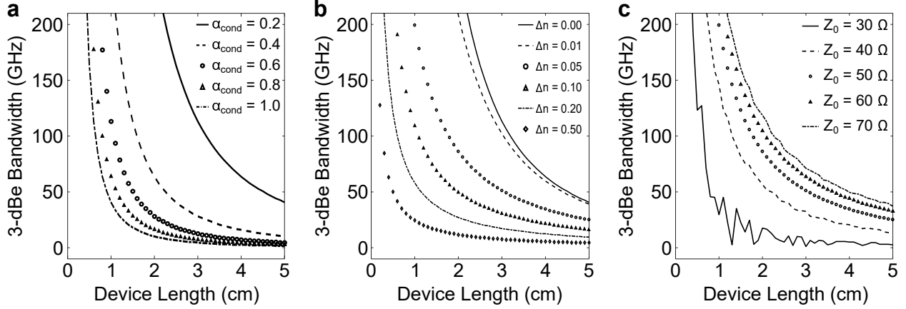
Figure 1.4: The results shown in this figure are simulated 3-dBe electrical bandwidth values, in GHz, based on Equation 1.23. a Assumes perfect index matching ( \Delta n = 0 ) and perfect impedance matching ( Z_G = Z_0 = Z_L = 50 \Omega ). Each curve represents a different electrical conductor loss ( \alpha_{cond} , the only significant source of electrical loss at high frequencies for a well-designed device), in units of dB/[cm-GHz 1/2 ]. b Different index matching values are shown for \alpha_{cond} = 0.2 dB/[cm-GHz 1/2 ] and perfect impedance matching. \Delta n = n_m - n_o . c In this case, \alpha_{cond} = 0.2 dB/[cm-GHz 1/2 ], \Delta n = 0.05 , and different values of Z_0 are plotted, assuming Z_G = Z_L = 50 \Omega .
