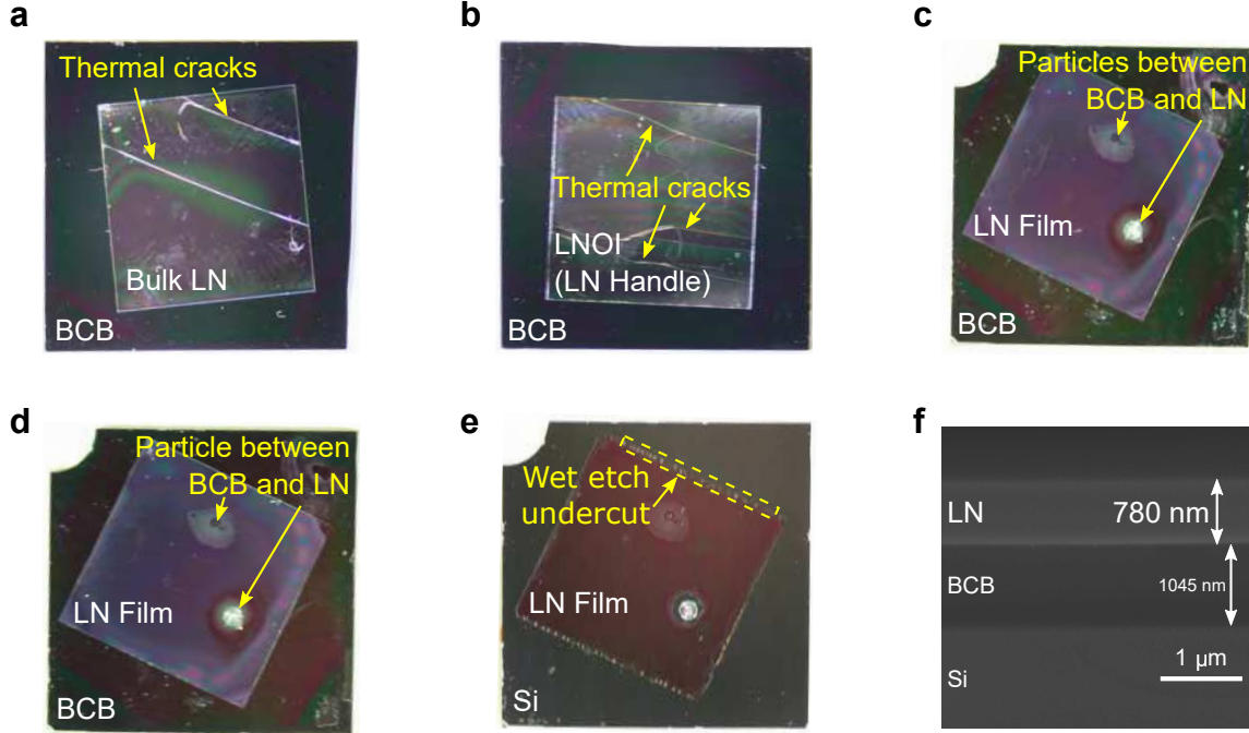
Figure 4.7: a through e show camera images of 1\text{ cm} \times 1\text{ cm} pieces of LN or LNOI which were bonded to bulk Si pieces of a similar size through a 1\text{ }\mu\text{m} BCB layer. a is bulk LN, b is LNOI with a LN handle, and c through e are LNOI with a Si handle, which has been removed by dry-etching (note that the \text{SiO}_2 layer is still on the LN film in c and d ). c shows the chip after substrate removal. d shows the same chip after 10 thermal cycles between room temperature and 300^\circ\text{C} . e shows the chip after the protective \text{SiO}_2 and surrounding BCB have been removed by respective HF and Piranha acid baths. A cross-section SEM image of e taken at an angle of 52^\circ from the vertical axis is presented in f , showing the \sim 1\text{ }\mu\text{m} thick BCB layer bonding a 780\text{ nm} thick film of LN to a bulk Si substrate.
